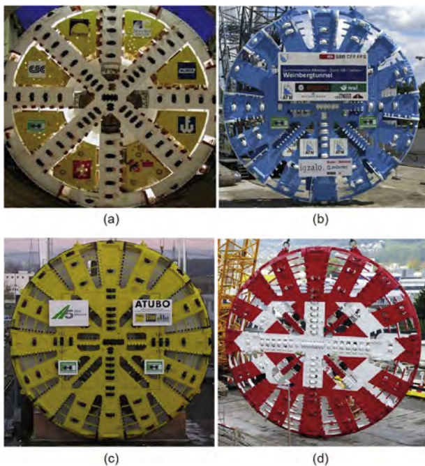
Fig. 2. Cutterheads for (a) the Zimmerberg base tunnel (1999) and the Oenzberg tunnel (2001), (b) the Weinberg tunnel (2008), (c) the Büntenberg tunnel and the Längholz tunnel (2008), and (d) the Eppenberg tunnel (2016).
