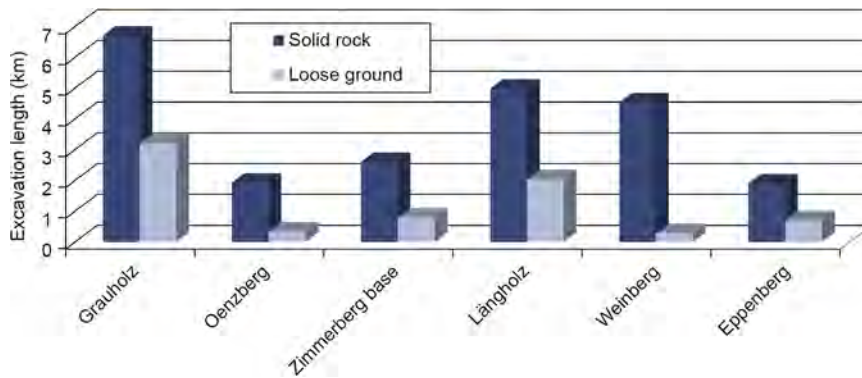
Fig. 1. Summary of TBM excavations in Switzerland with a large diameter (>10 m), loose ground sections, and necessary full-face support.
